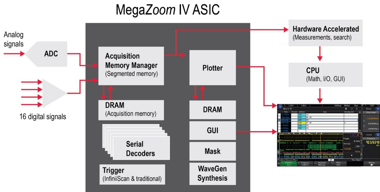
Figure 11. The 3000T X-Series oscilloscopes' uncompromised responsiveness, speed and waveform update rate are enabled by the MegaZoom IV, smart memory ASIC. The CPU is not used for core waveform operations.
