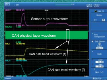
Example: Comparison and verification of actually measured signals and CAN bus signals
