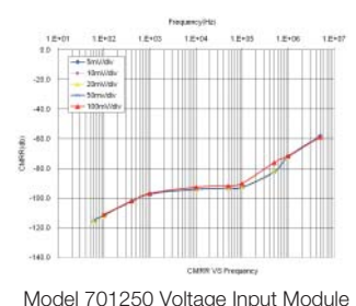
Model 701250 Voltage Input Module
