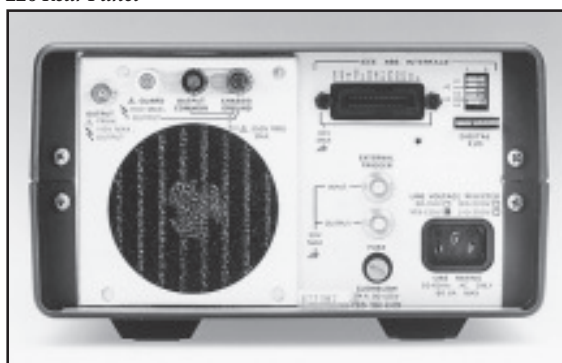
220 Rear Panel
