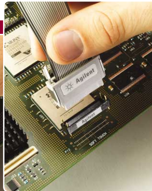
Figure 10. Soft touch connectorless probes have 1/4 the capacitive loading of connector probes and are the industry's most reliable connectorless solution.
