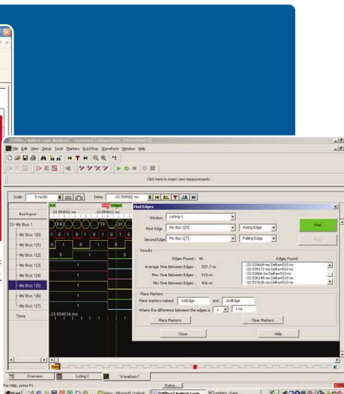
Figure 25. Extend your measurement results with customized data analysis.
