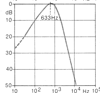
CCITT Rec. G. 227 Filter Option SUF 2-Z7
