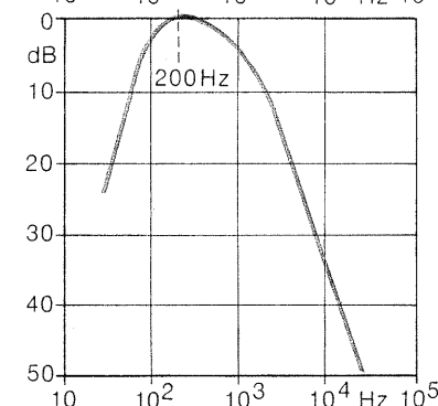
CCIR Rec. 559 Filter Option SUF 2-Z4
