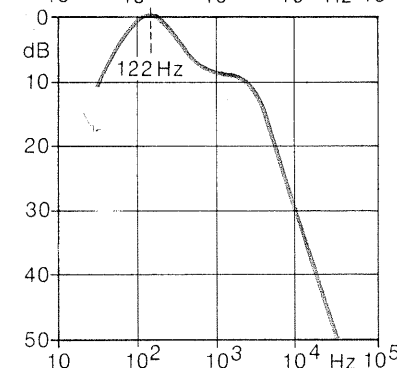
CCIR Rec. 571 Filter Option SUF 2-Z5
