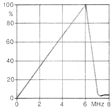
Triangular Noise Option SUF 2-Z2
