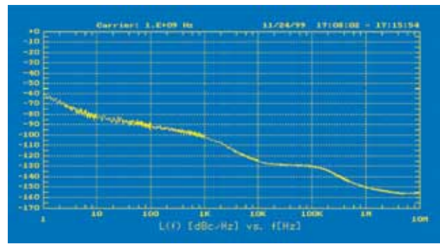
Typical SSB noise at 1 GHz (with OCXO option R&S SML-B1)
