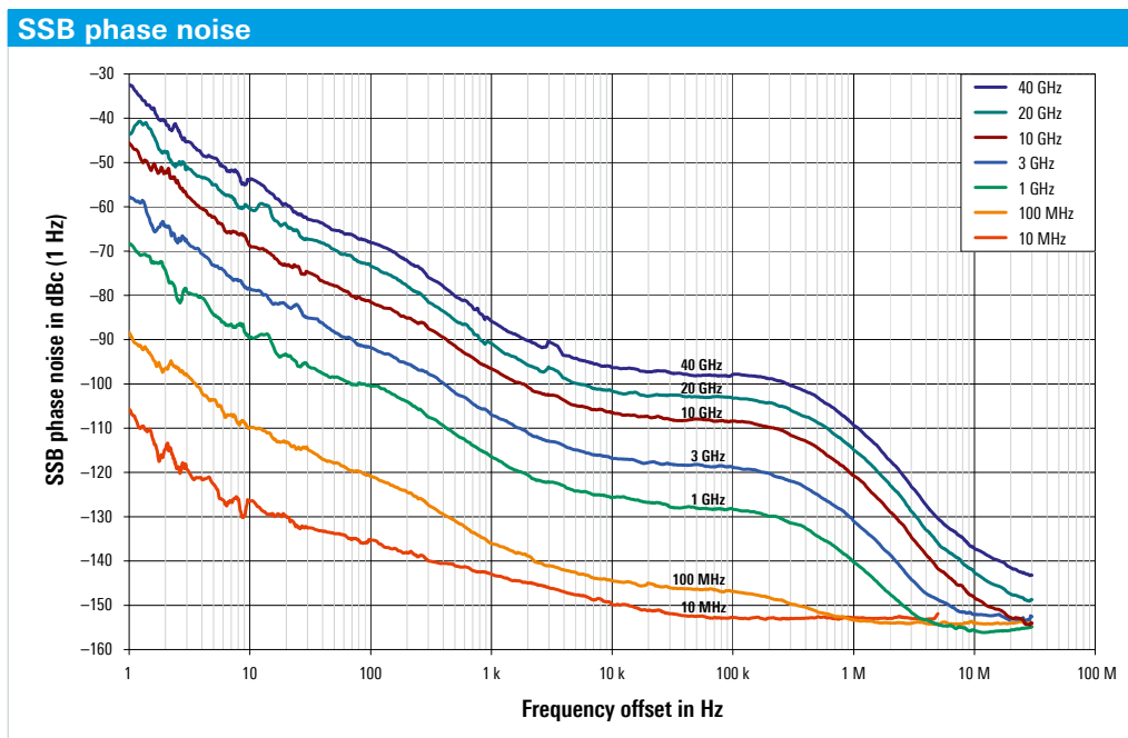
Measured SSB phase noise with the R&S®SMB-B1H OCXO option.
