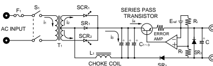
Fig. 5 Basic Circuitry of the PAD-L Series
