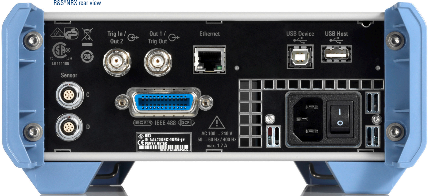
R&S®NRX rear view
