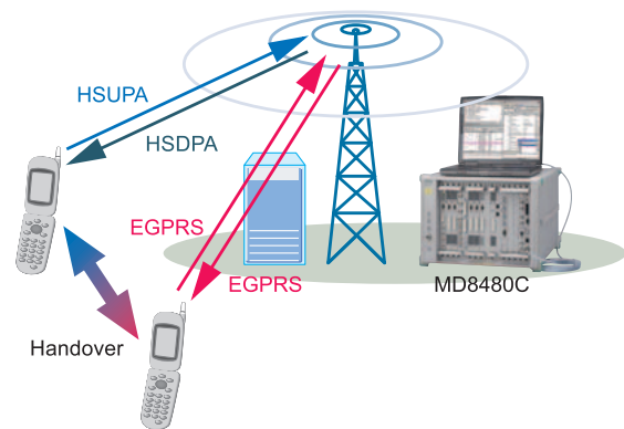
EGPRS-HSPA Handover Test
