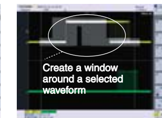
Waveform window search Select a waveform in History Memory and create a window around the waveform by moving up/down/left/right from the waveform. Search for waveforms that fall inside or outside the window.
