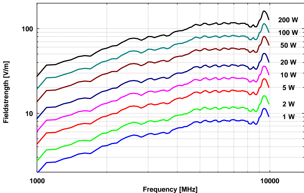
BBHA 9120 B Input Power, Dist. Aperture-EuT: 4 m
