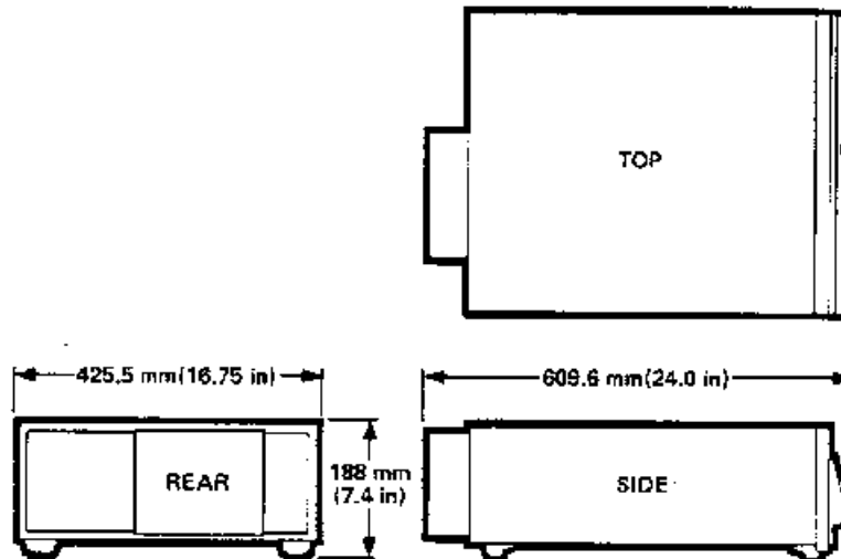
Figure 6. Instrument Dimensions
