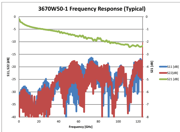
3670W50-1 Frequency Response (Typical)
