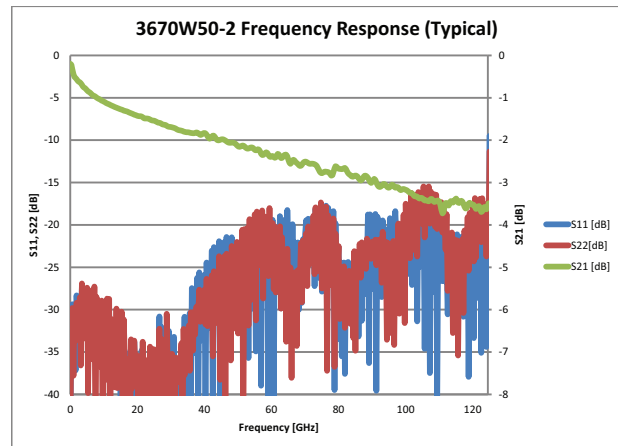
3670W50-2 Frequency Response (Typical)
