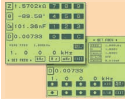
Measurement frequency Use the numeric keypad or digit keys to enter the setting values, changing the test frequency or level while monitoring the measurement. The level setting can be open-circuit voltage, constant voltage, or constant current.
