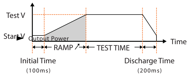
Output Voltage Variation in One Test Cycle
