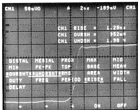
The auto measure feature provides a menu of the 21 measurements that you can select. Here the user selected rise time, undershoot, and overshoot measurements of the waveform on channel 1.
