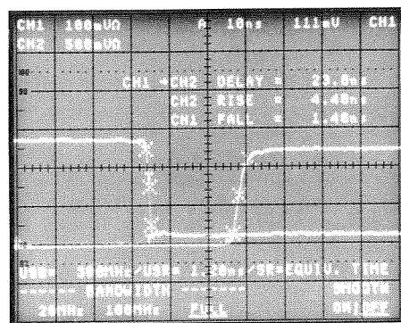
Here, a 2440 user has set markers and selected propagation delay, rise time and fall time measurements—all by simply pressing a few front panel buttons.
