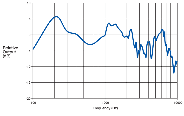
Figure 3. Frequency Response
