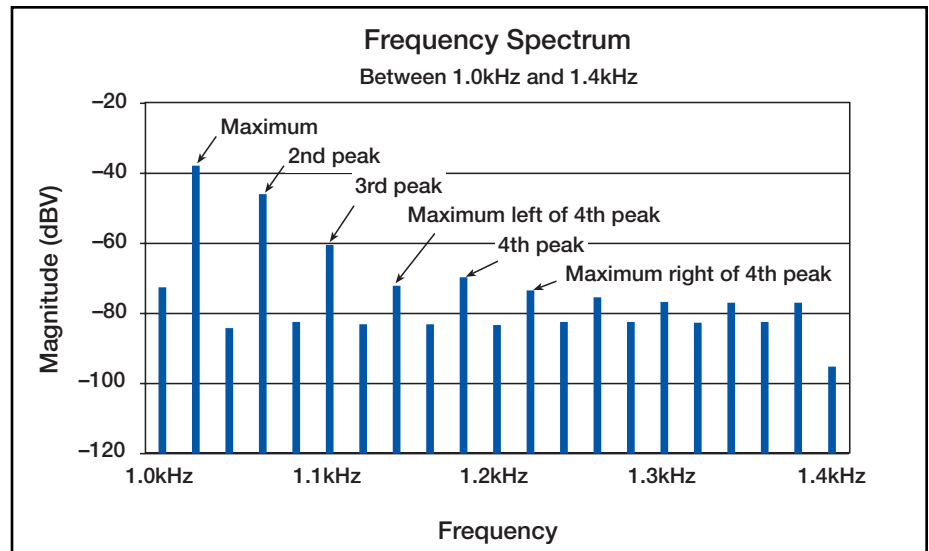
Figure 4. The Model 2015-P directly identifies peak values of the frequency spectrum.
