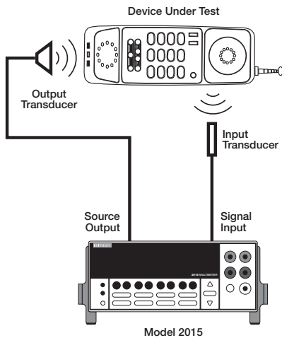
Figure 1. Total Harmonic Distortion Analysis and Frequency Response of a Portable Wireless Telecommunication Device
