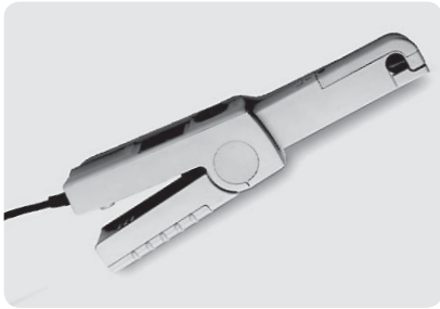
1146A 100 mA to 100 Arms, dc to 100 kHz probe.
