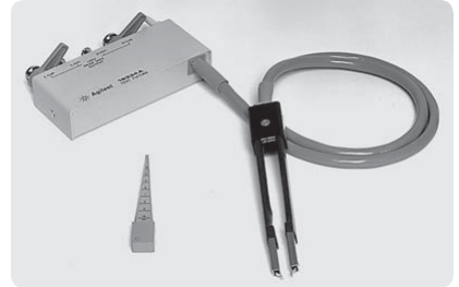
16334A SMD/chip tweezers Frequency: \leq 15 MHz Maximum dc bias: \pm 42 V
