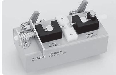
16034G small SMD/chip test fixture Frequency: \leq 110 MHz Maximum dc bias: \pm 40 V
