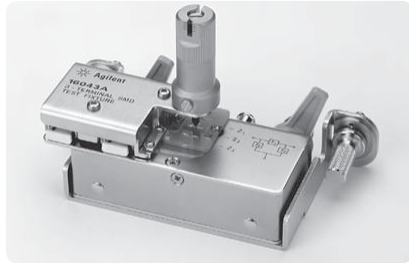
16043-60011 test fixture 16043-60012 test fixture Frequency: \leq 110 MHz Maximum dc bias: \pm 40 V
