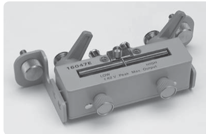
16047E test fixture Frequency: \leq 110 MHz Maximum dc bias: \pm 40 V
