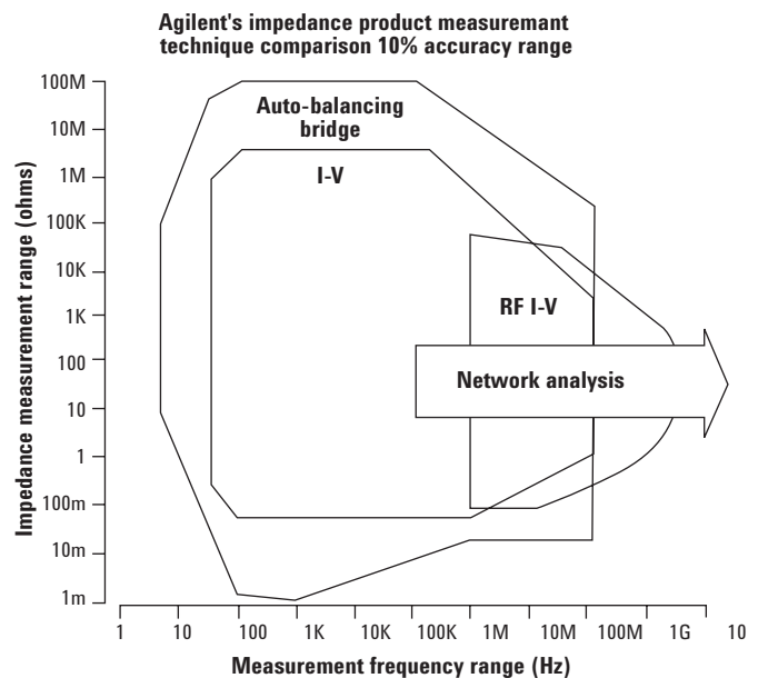
Figure 1. Impedance measurement technique
