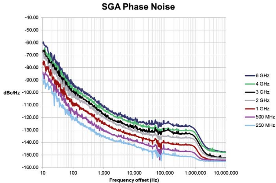
Graph of typical phase noise performance
