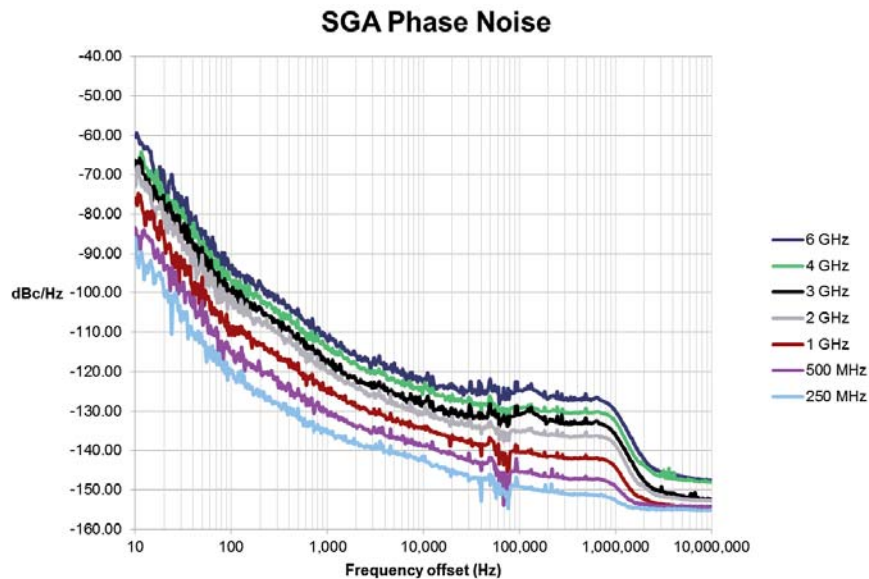
Typical phase noise performance at 250 MHz, 500 MHz, 1 GHz, 2 GHz, 3 GHz, 4 GHz and 6 GHz
