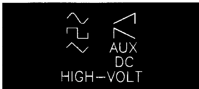
The HP 3324A offers 5 standard waveforms, an Auxiliary TTL clock and DC. The standard waveforms and DC can be combined with the High-Voltage Output Option.
