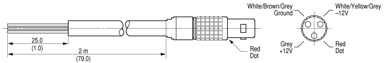
83006-60004 dc bias cable. Cable shipped with 83006A, 83017A, 83018A, 83050A, and 83051A.
