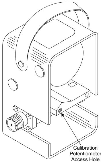
Figure 10 Calibration Potentiometer
