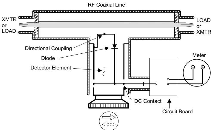
Figure 1 Element Schematic Diagram
