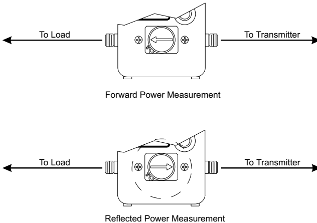
Figure 5 Measurement Direction
