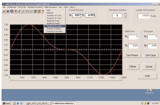
Fig1 Arbitrary Waveform Generation Software
