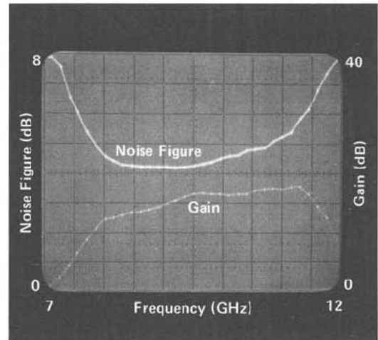
Typical oscilloscope display of amplifier.
